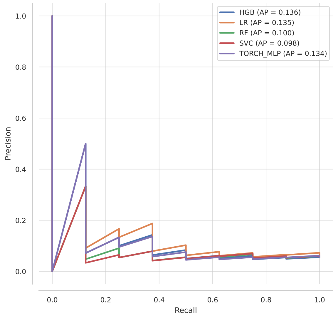
Combined PR Curve (Severe complication)
